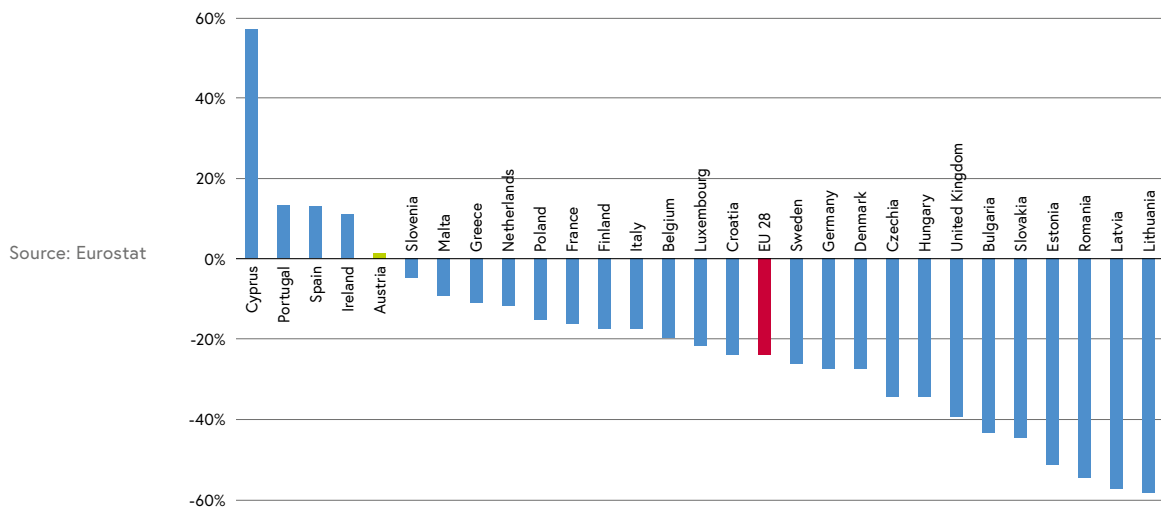
Figure 1: Greenhouse gas emissions of the EU 28 countries in relation to the level of 1990 [%]
