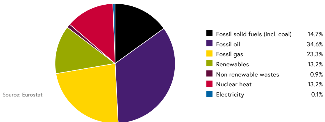
Figure 9: Structure of gross inland energy consumption of the EU 28 countries in 2016 [%], in total 68689 PJ
