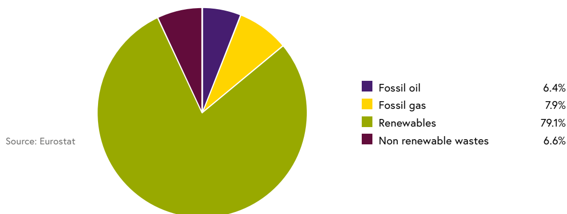
Figure 14: Structure of primary energy production of Austria in 2016 [%], in total 517 PJ
