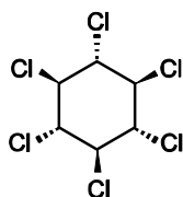
beta-HCH
