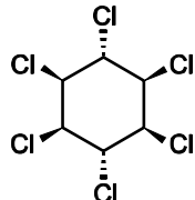
Lindane (gamma-HCH)
