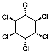
alpha-HCH
